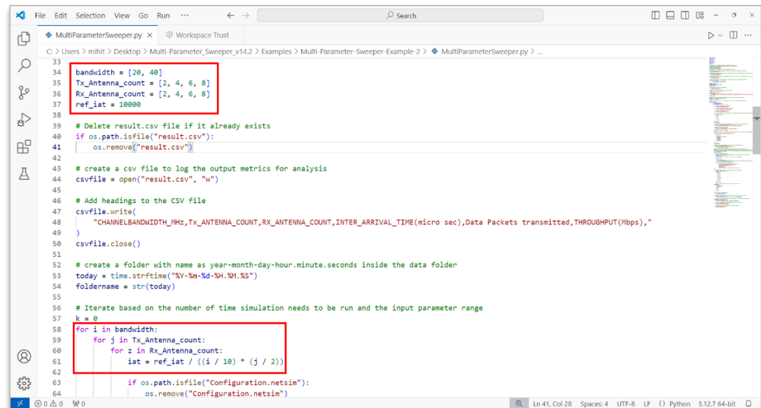
Figure 28: Modified MultiParameterSweeper.py based on input parameter
