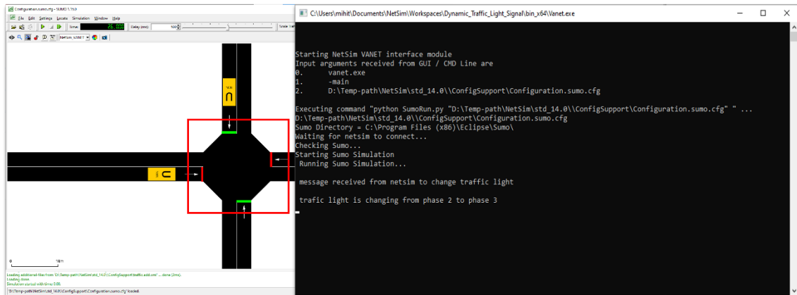
Figure 4: Control Message received from NetSim
