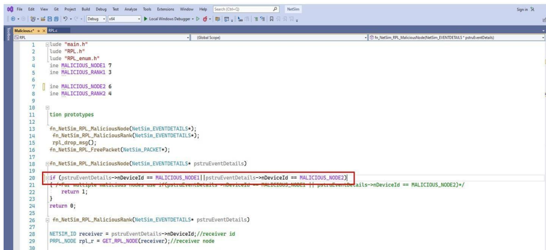
Figure 7: If condition for checking multiple malicious nodes 5.
