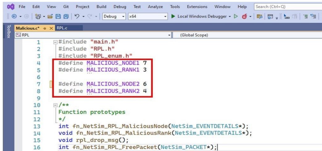
Figure 6: Defining malicious nodes in Malicious.c file
