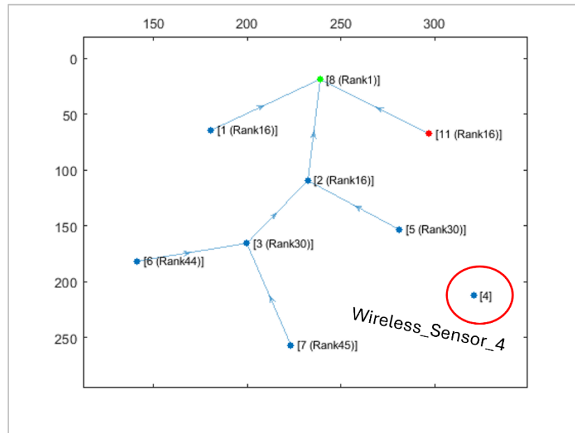
Figure 6: DODAG Formation Graph from MATLAB
