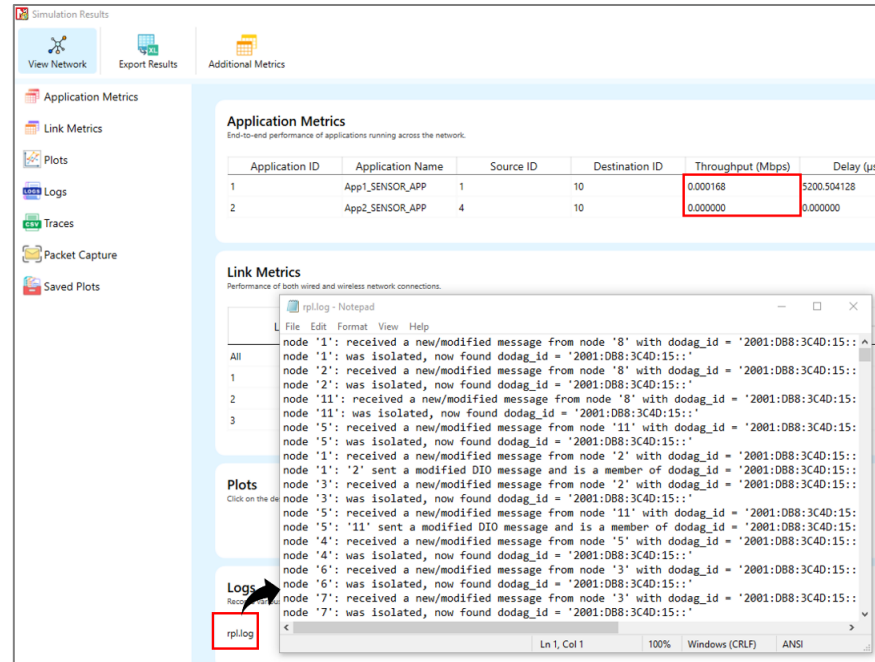
Figure 9: NetSim Results Dashboard Window
