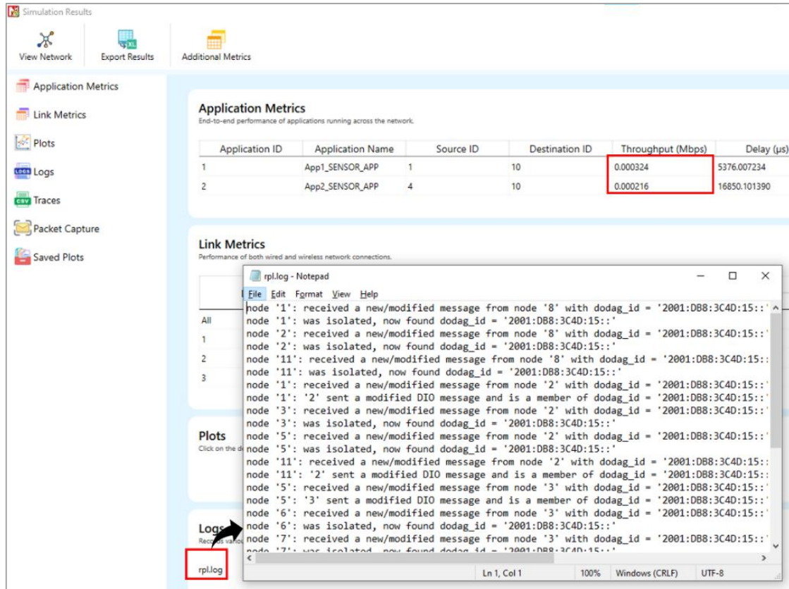
Figure 7: NetSim results dashboard
