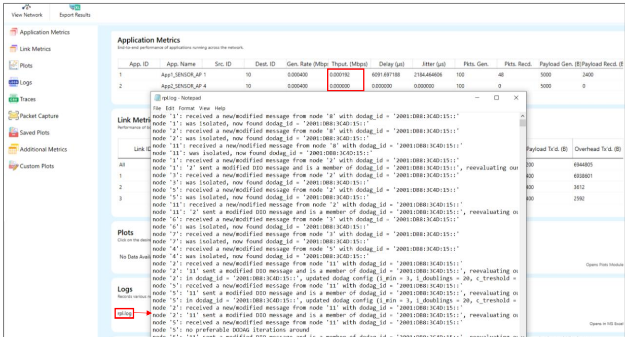
Figure 5: NetSim results dashboard
