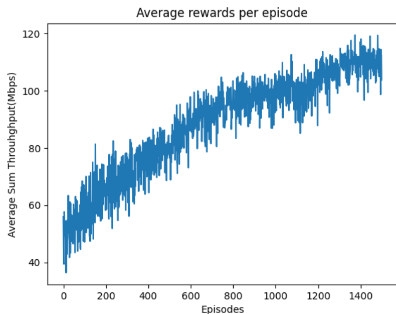
Average rewards vs episode count
