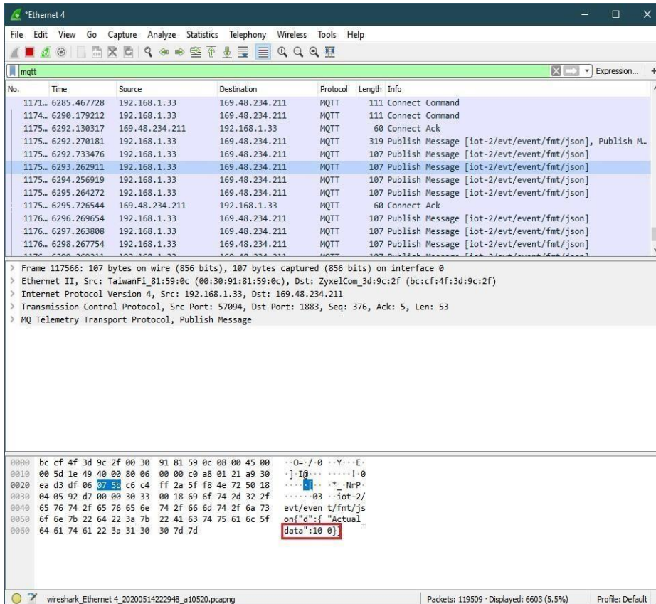
Figure Wireshark
