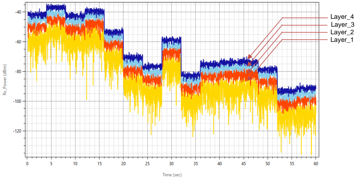
Rx_Power_GNB_7_IF4_UE_10_IF1_CA1_LAYERS_4_DL
