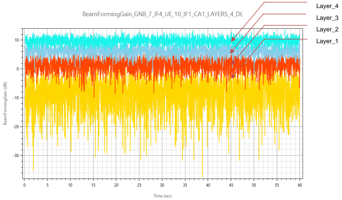
Figure 8: Beam Forming Gain in NetSim
