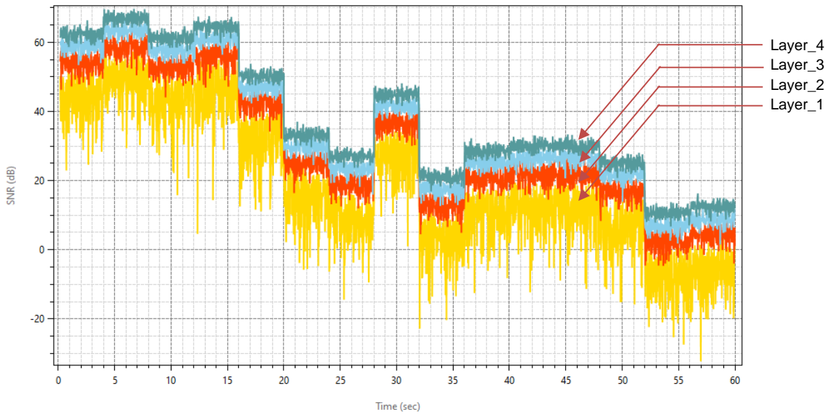
SNR_GNB_7_IF4_UE_10_IF1_CA1_LAYERS_4_DL
