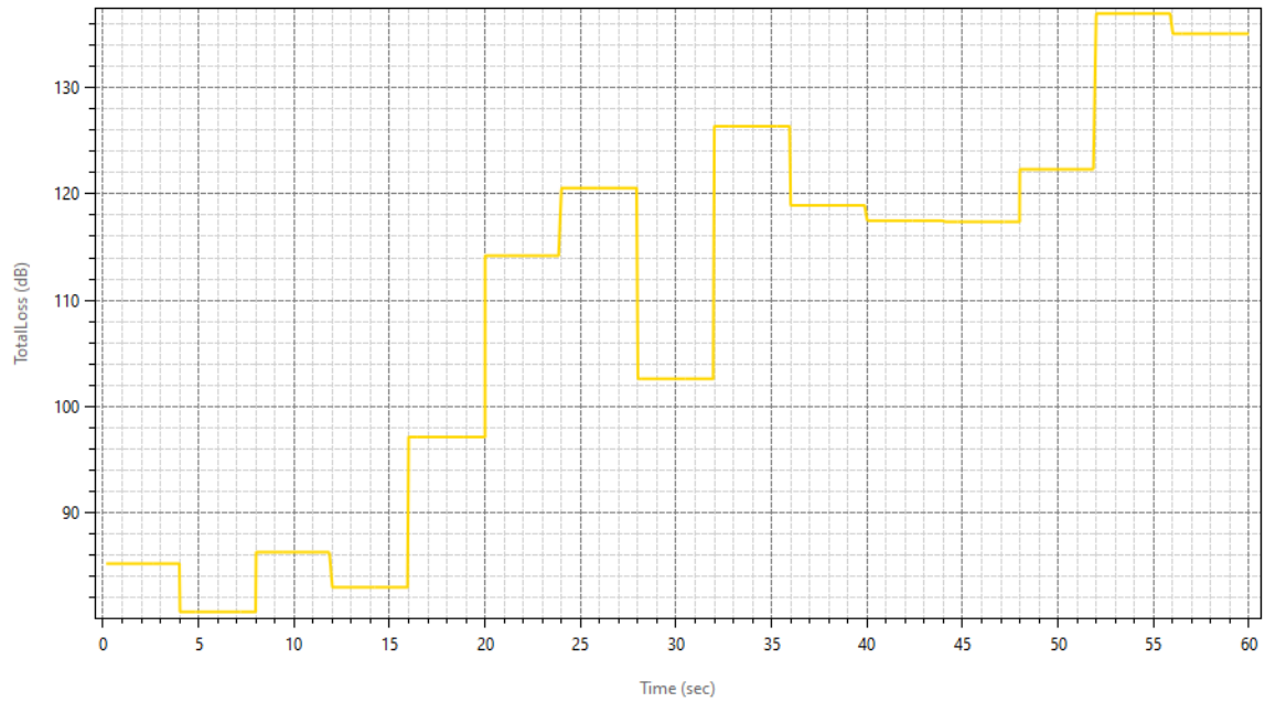
TotalLoss_GNB_7_IF4_UE_10_IF1_CA1
