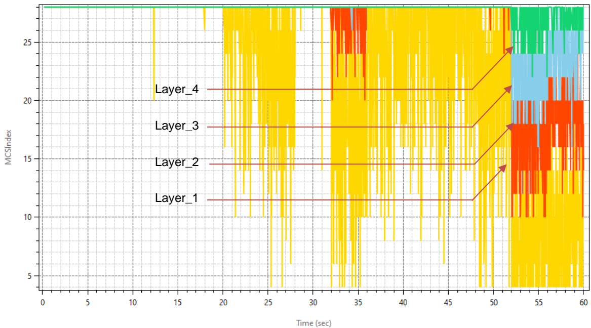
MCSIndex_GNB_7_IF4_UE_10_IF1_CA1_LAYERS_4_DL
