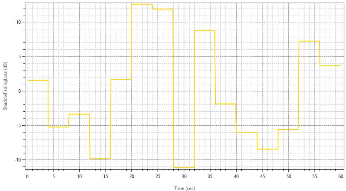
ShadowFadingLoss_GNB_7>If_4_UE_10>If_1_CA_1
