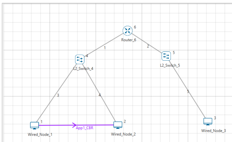
Figure 1-3: Network set up for studying the ARP across a LAN
