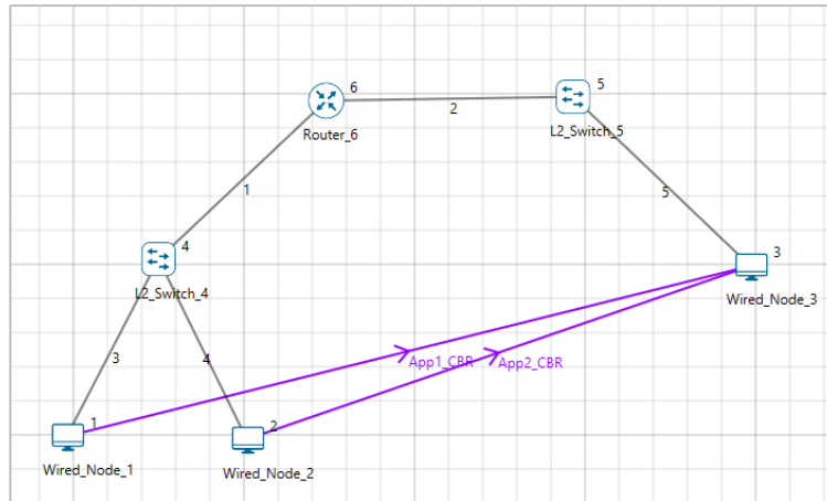
Figure 1-7: Network set up for studying the ARP across a WAN
