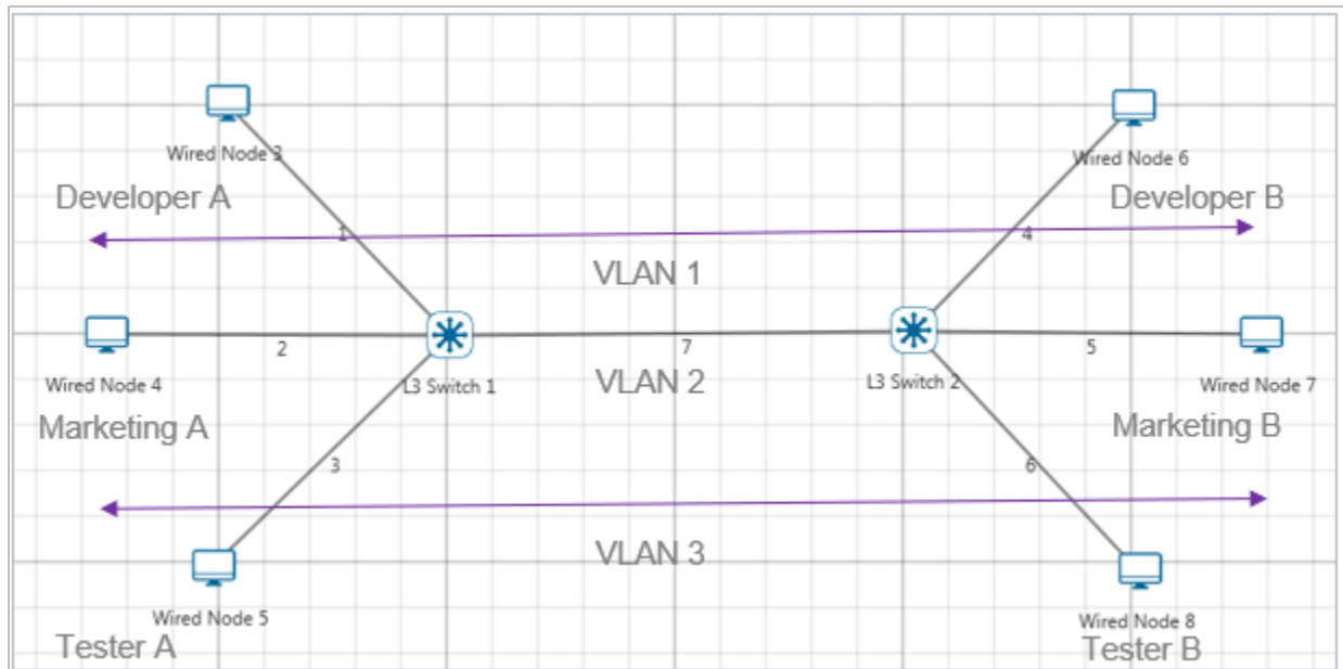
Figure 1-2: Hosts in one VLAN need to communicate with hosts in another VLAN This is known as Inter-VLAN routing
