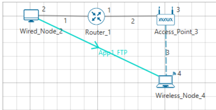
Figure 1-2: Network set up for studying the WiFi Network with Single TCP Download
