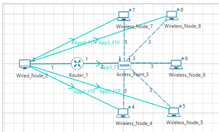
Figure 1-4: WiFi Network with Multiple TCP Download
