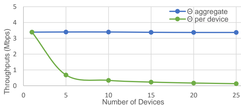
Figure 1-5: Plot of Number of devices vs. Throughputs (Mbps)
