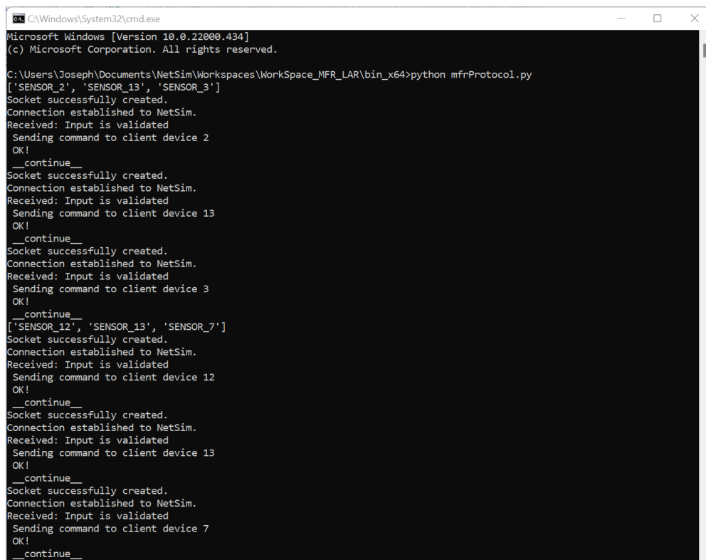
Figure 6: Python interface interacts with NetSim Simulation
