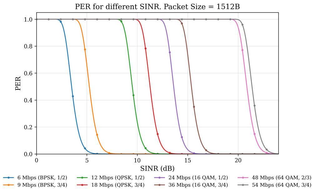
Figure 6-1: PER – SINR Combined Curve for all PHY rates
